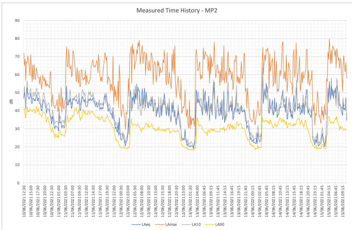
FIGURE 9: MP2 - MEASURED TIME HISTORY
