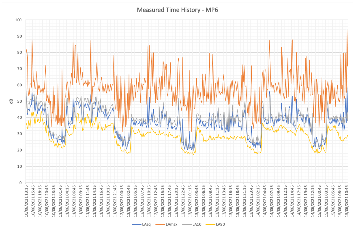
FIGURE 21: MP6 - MEASURED TIME HISTORY
