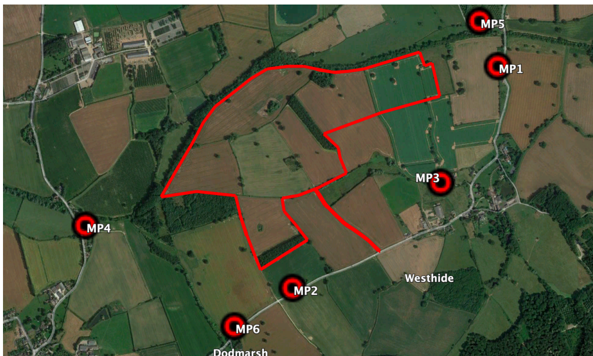
FIGURE 3: MEASUREMENT POSITIONS
