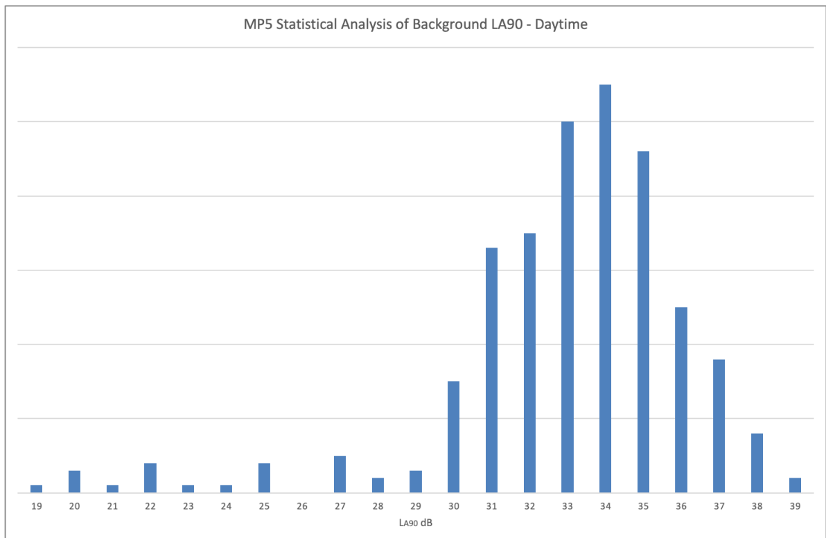
FIGURE 19: MP5 - STATISTICAL ANALYSIS OF LA90 BACKGROUND - DAYTIME
