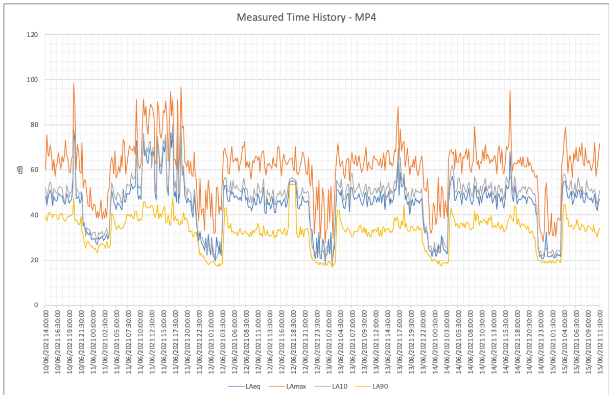
FIGURE 15: MP4 - MEASURED TIME HISTORY
