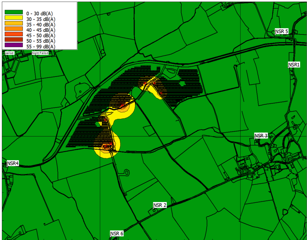
FIGURE 5: SPECIFIC SOUND LEVEL MAP (NIGHT-TIME)
